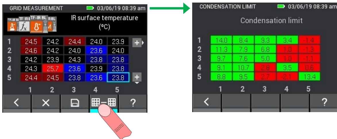
Figure 8-26: Special function of the TF-IR BL shows difference between surface temperature and dew point temperature
